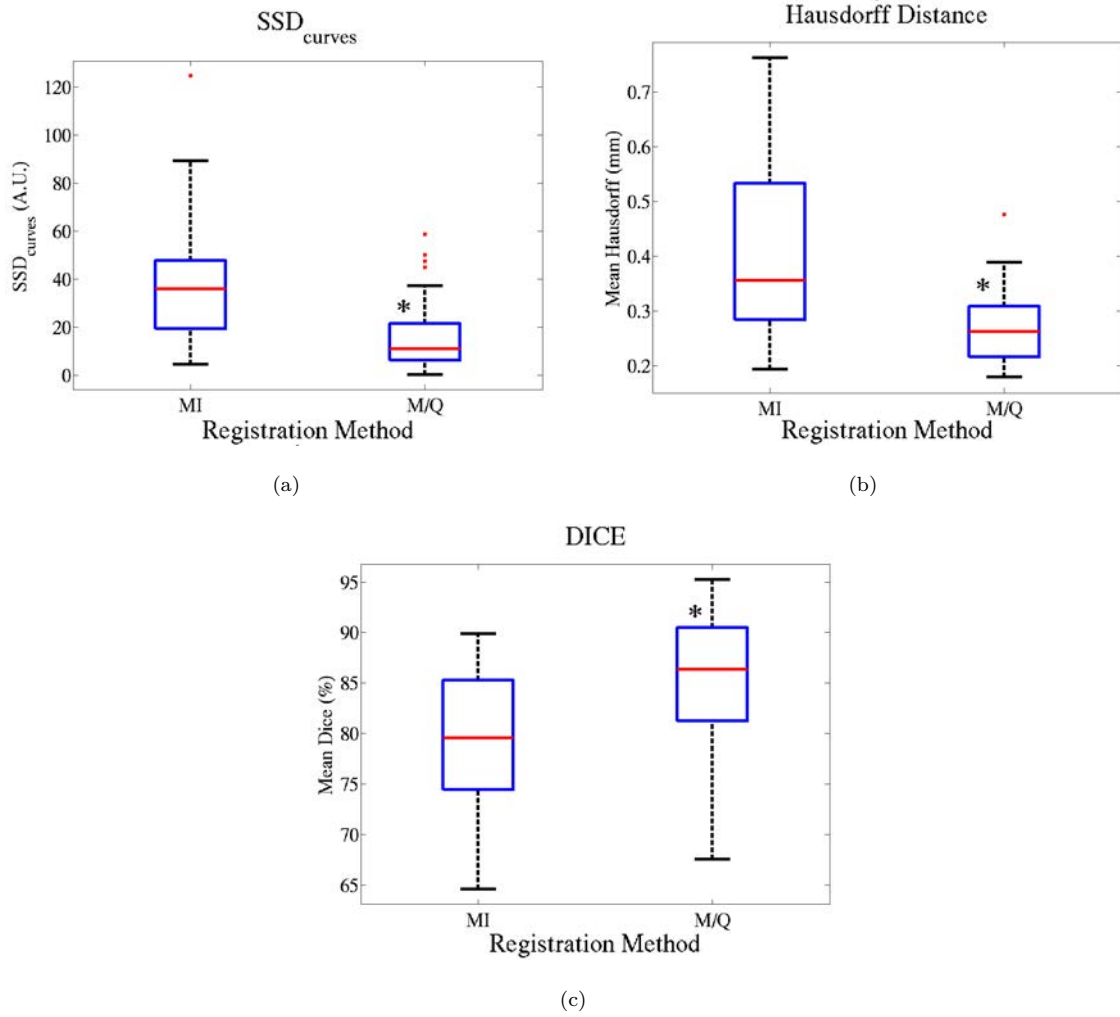
Figure 5.2: Boxplots of the distribution of the results for simulated sequences, for three criteria. a) SSD_{curves} b) Hausdorff distance c) DICE coefficient
