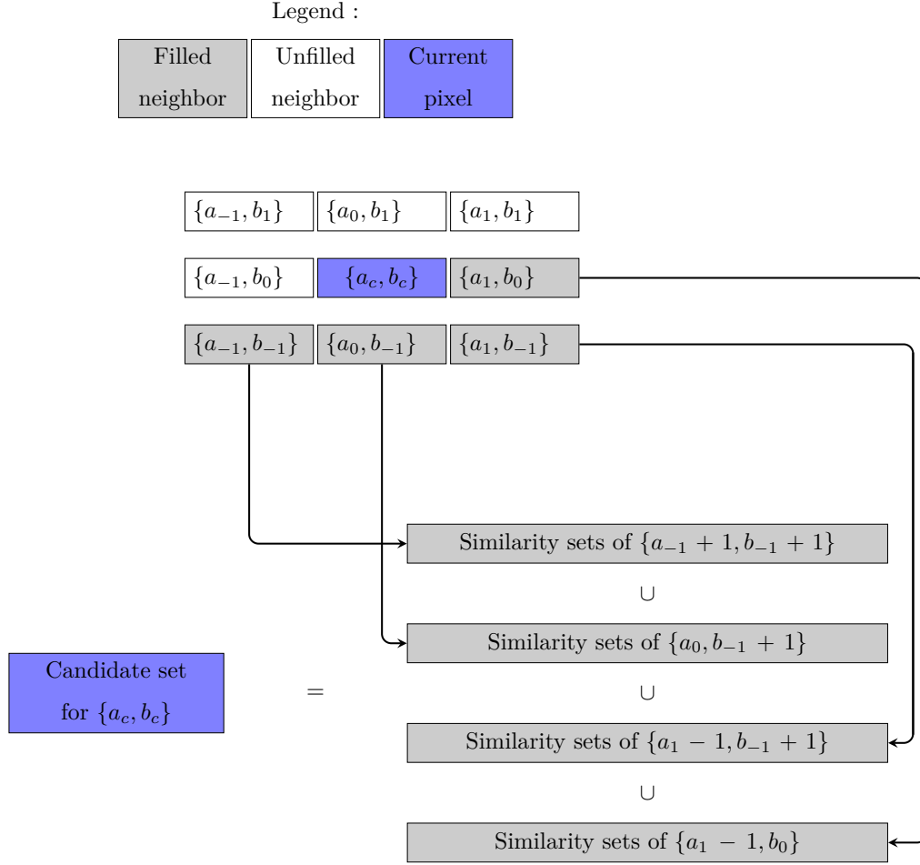
Figure A.1: Schematic diagram of an example of the synthesis phase. For each pixel, the original coordinates of the pixel in the sample are shown in brackets. \{a_c, b_c\} is unknown and needs to be determined. The candidate set is constituted according to the position of the neighbors in the original sample image. After the end of the synthesis phase for this pixel, the algorithm will go to the next unfilled pixel which, in this case, will be pixel \{a_{-1}, b_0\} .
